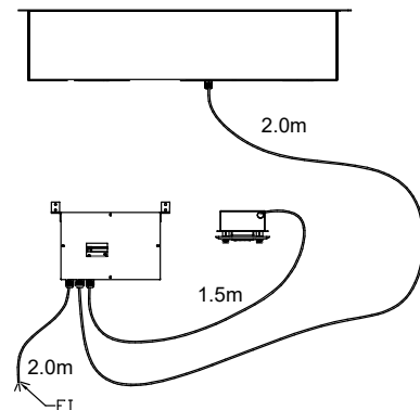
595T01M00 - WATER BAIN MARIE SEPARATED WELLS
